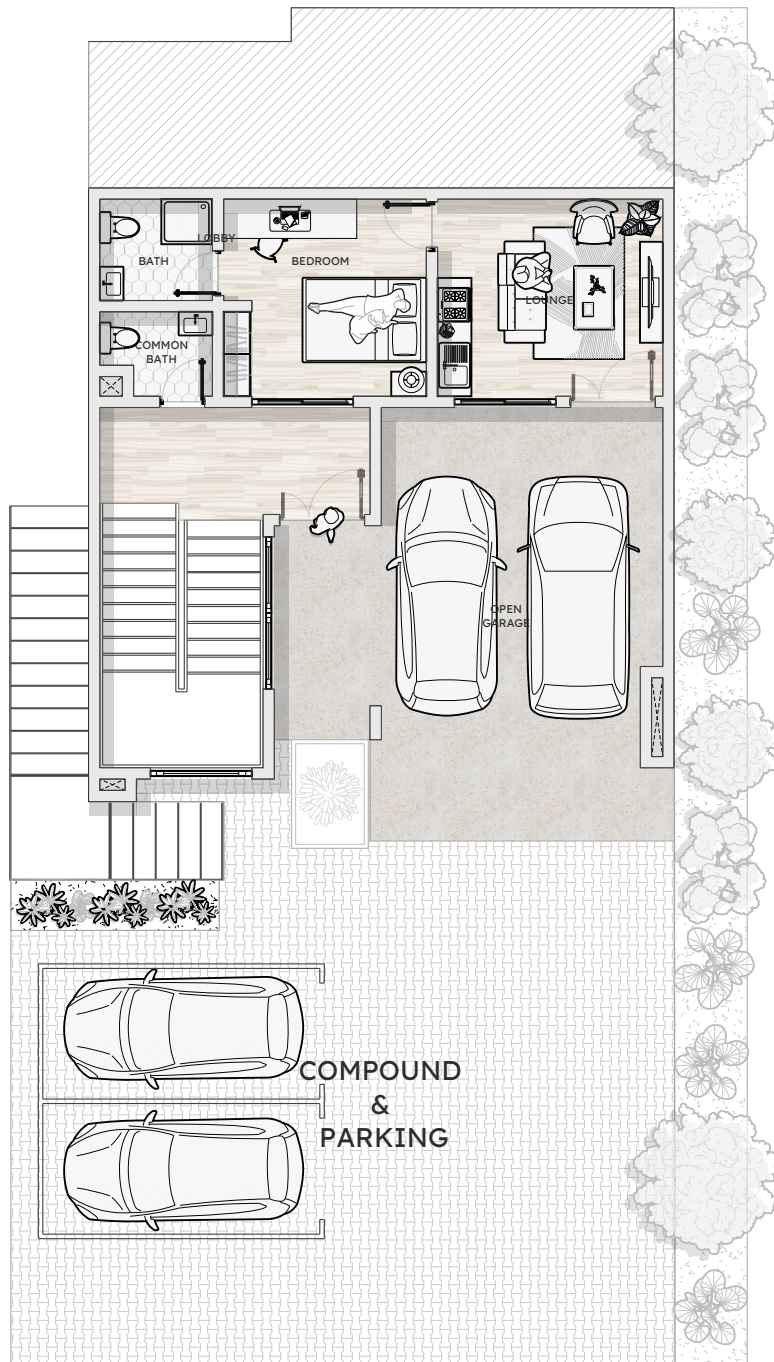
LOWER GROUND FLOOR PLAN
